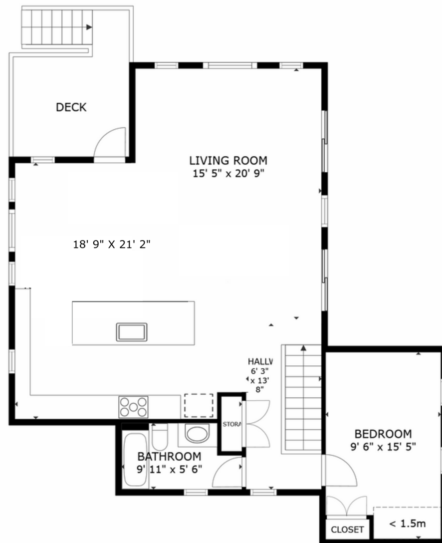
Second Floor
