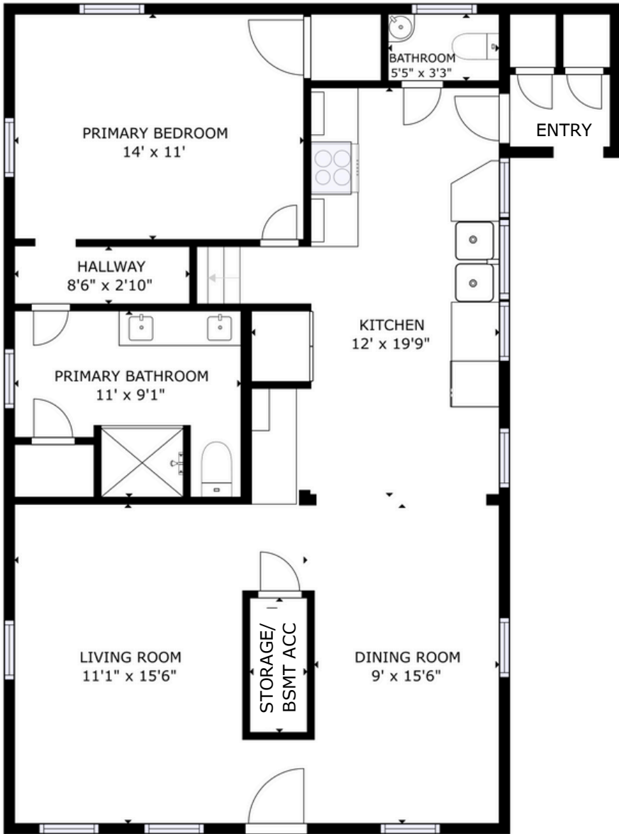
First Floor
