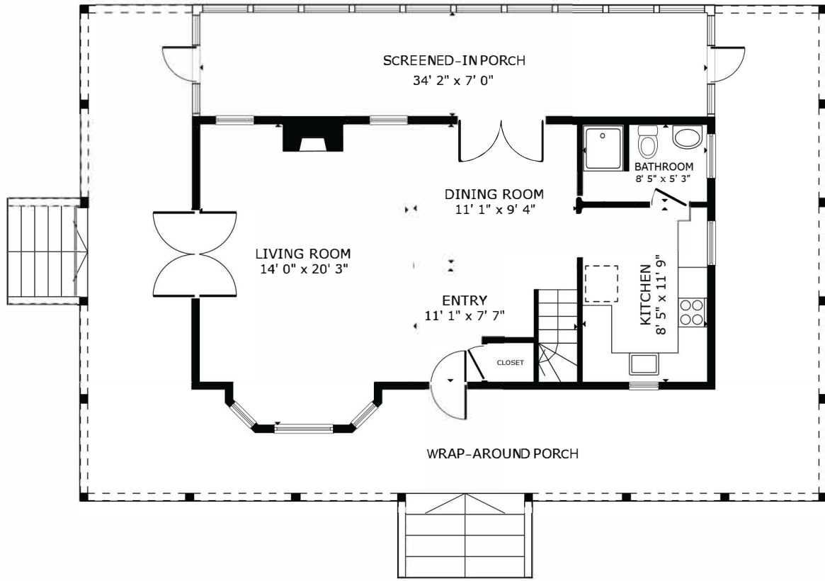
FLOOR 1
