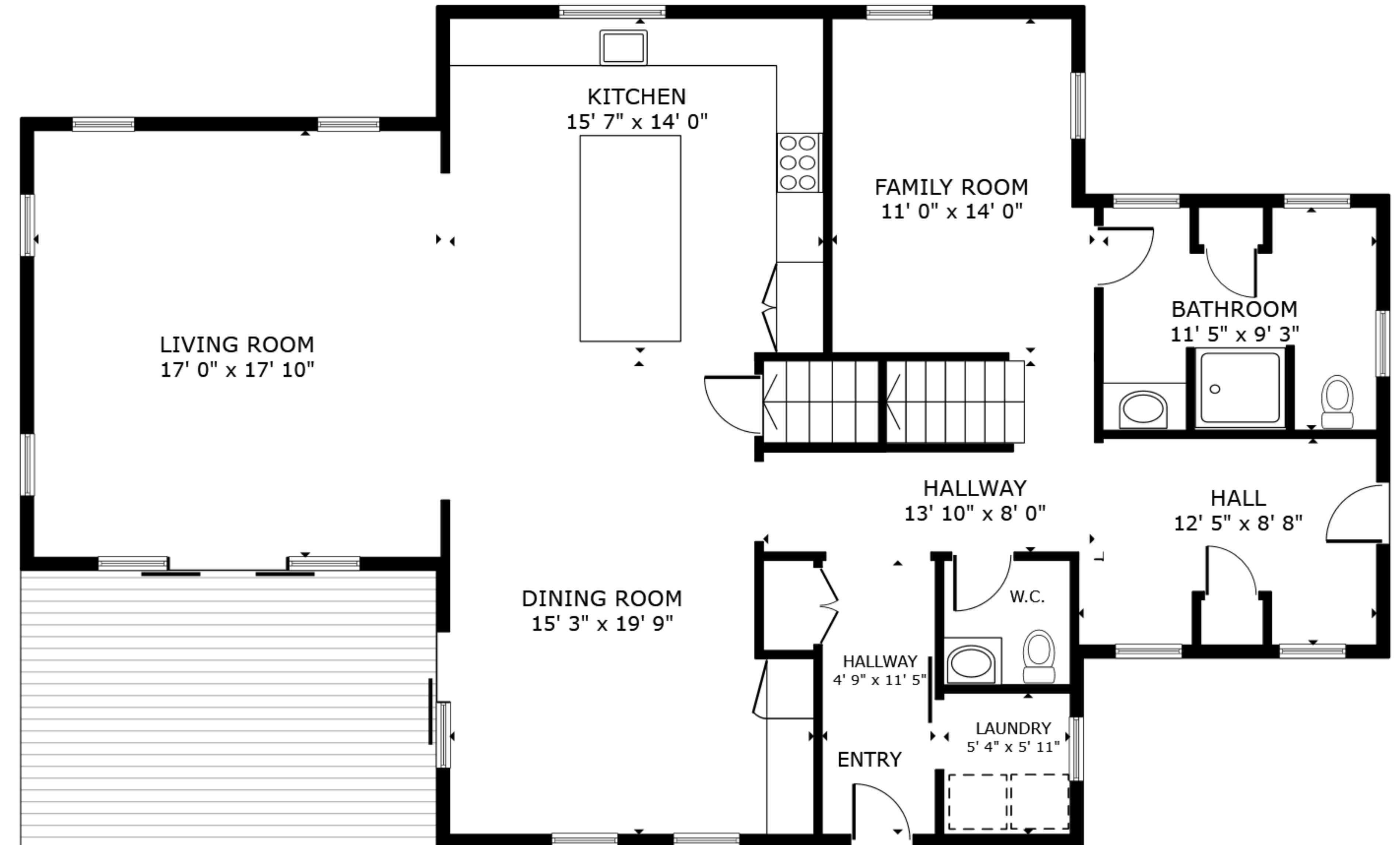
FIRST FLOOR
