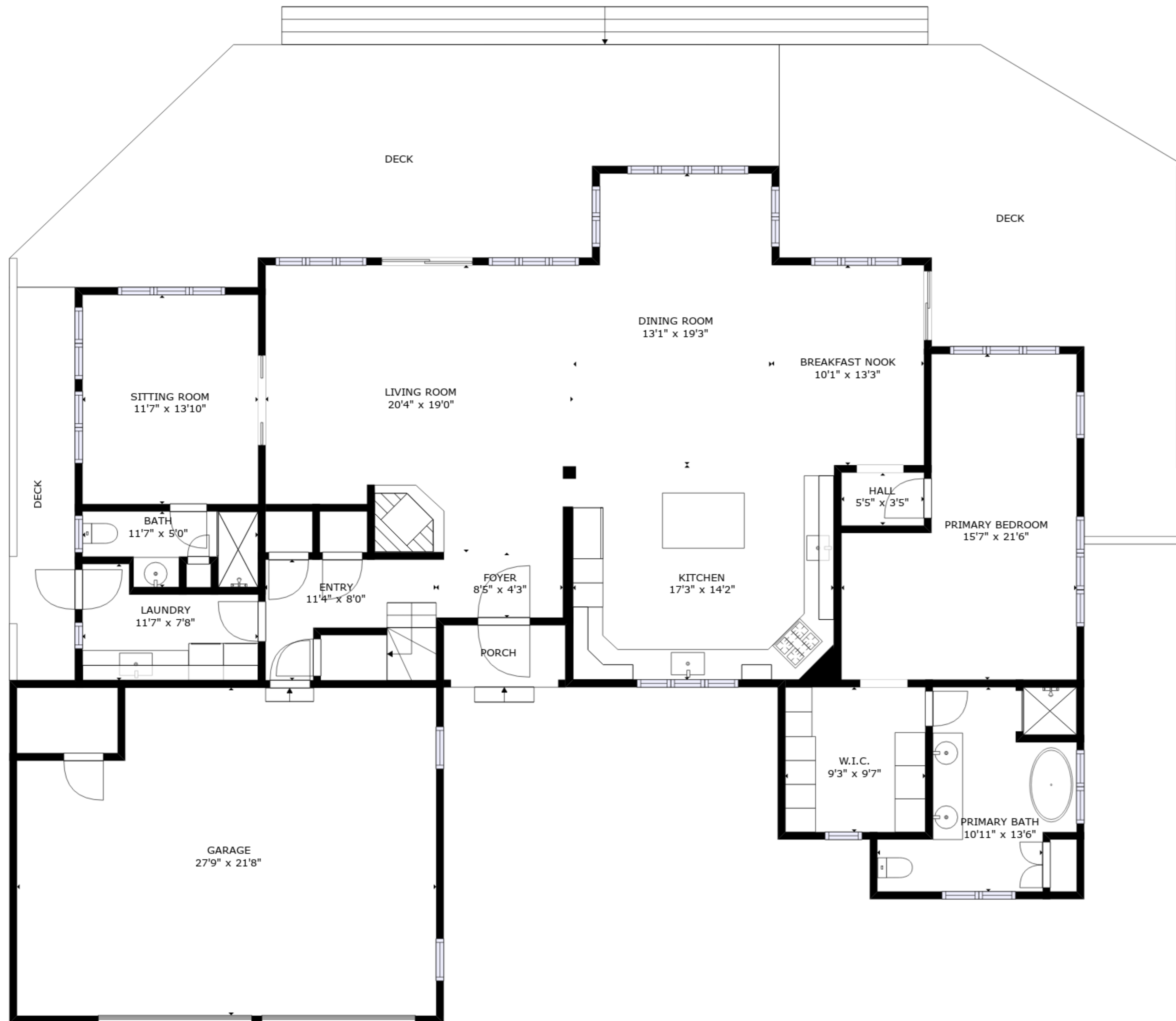
FLOOR 1
