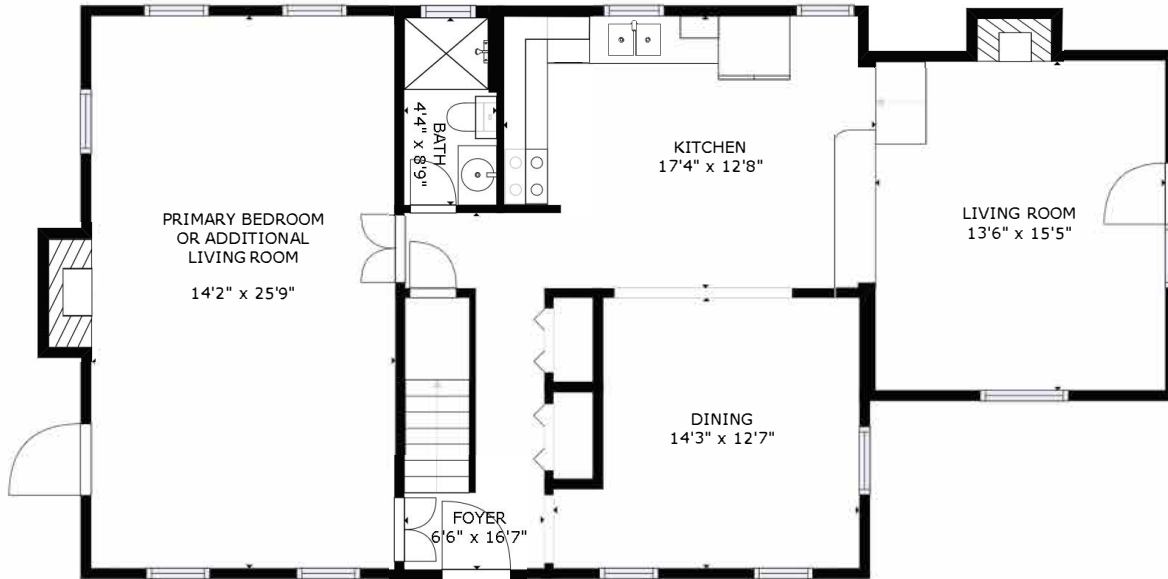
FLOOR 1
