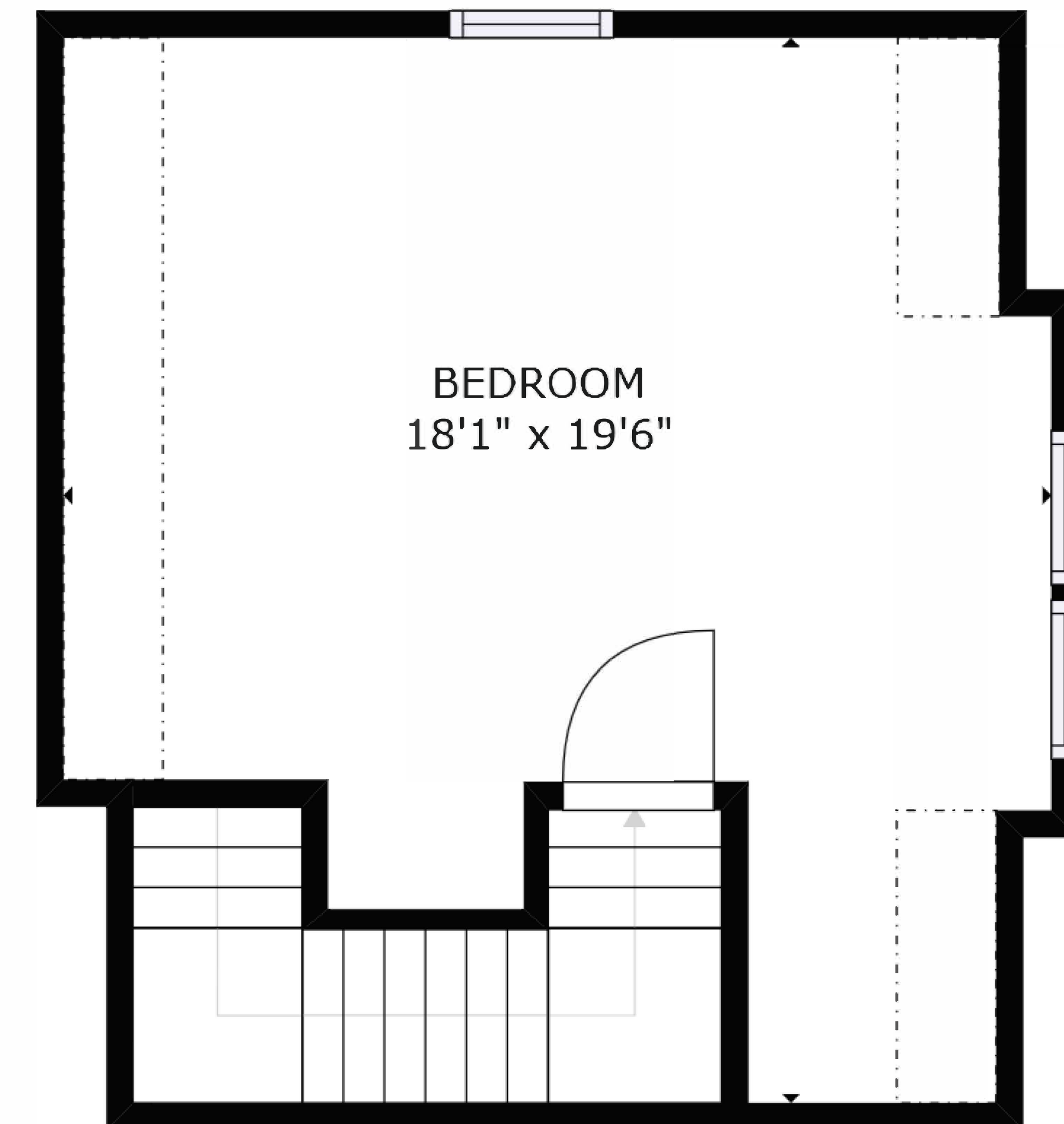
FLOOR 3
